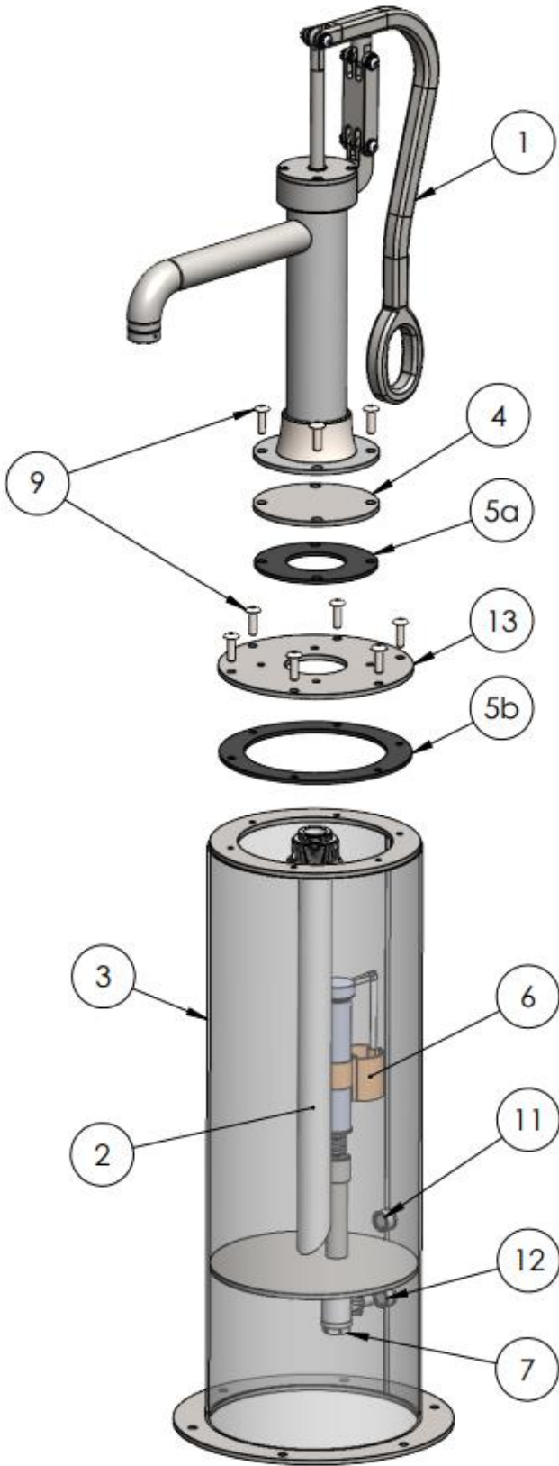
DIAGRAM B: Pump-n-Play Exploded View
